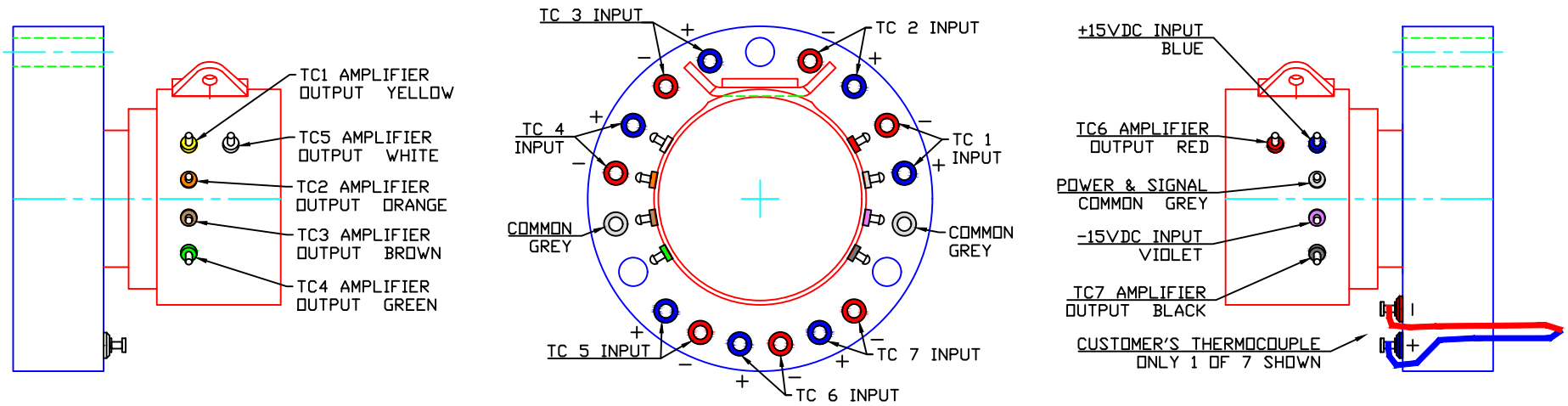
BLOCK DIAGRAM WITH MICHIGAN SCIENTIFIC PS-DC OR PS-DC
